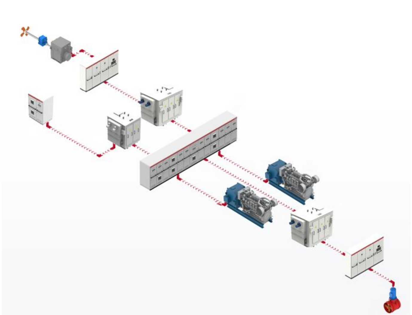
Diesel-Electric Propulsion System
