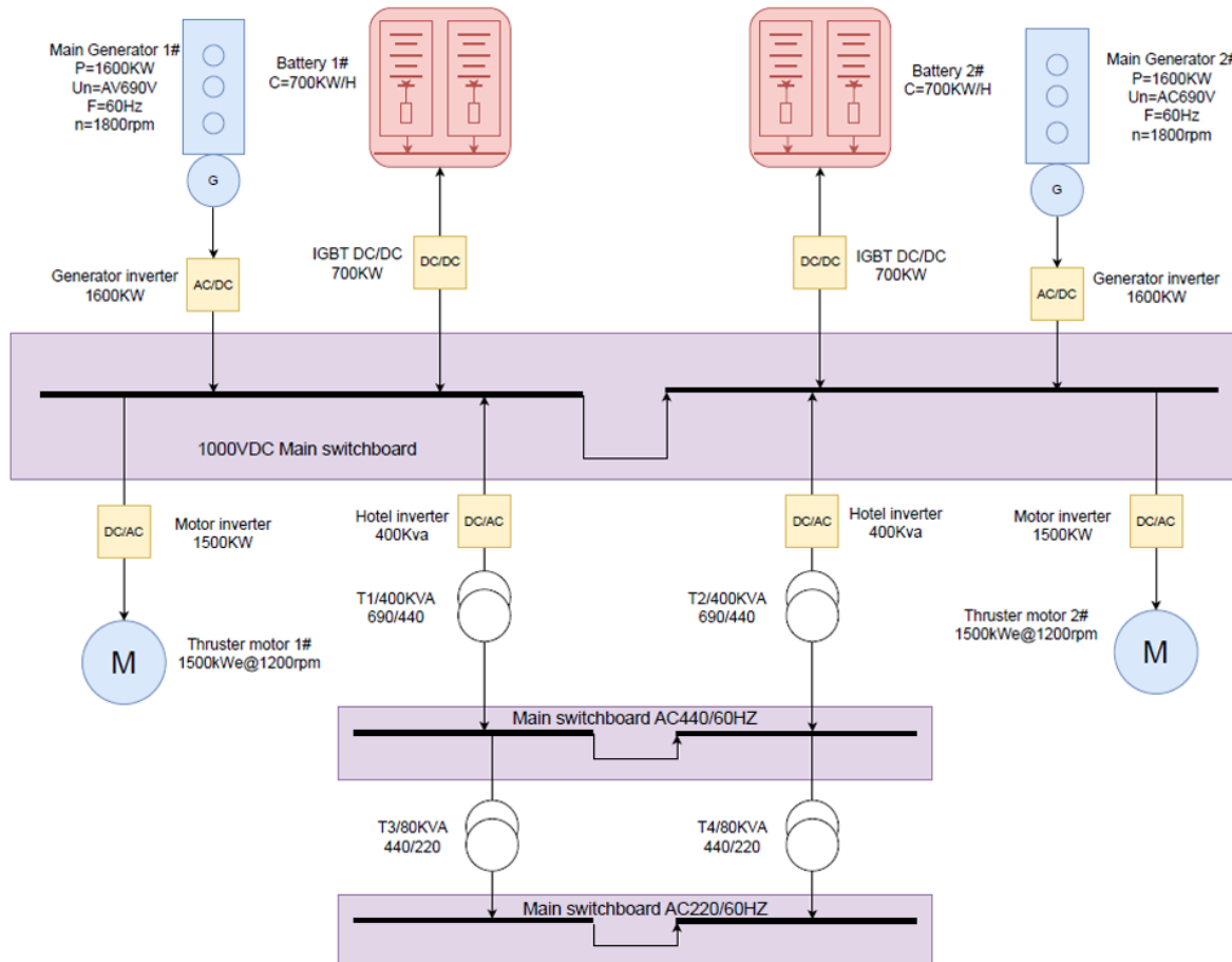
4000HP Hybrid Tugboat
